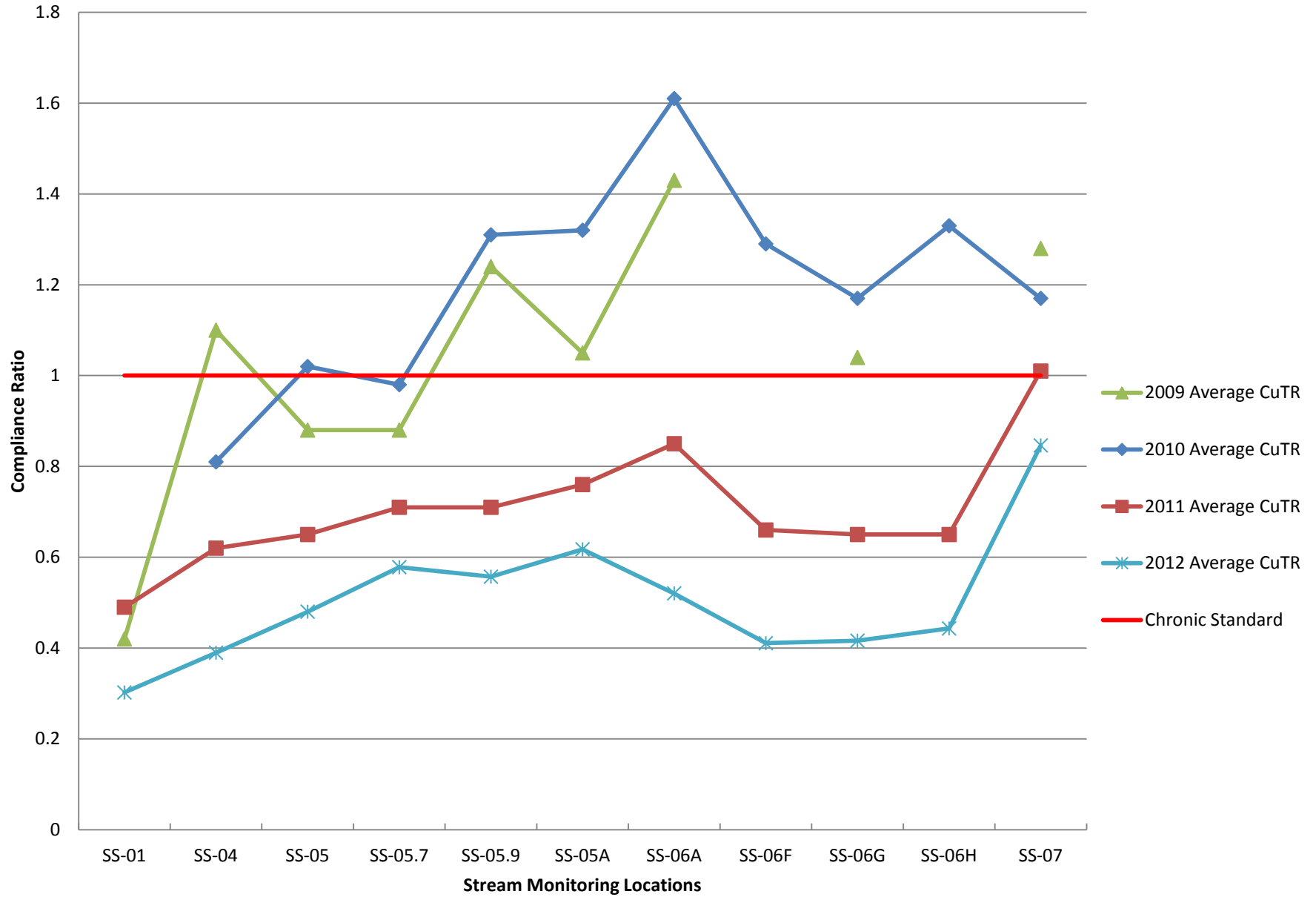
2009-2012 Total Recoverable Average Copper Compliance Ratios (Base Flow)
